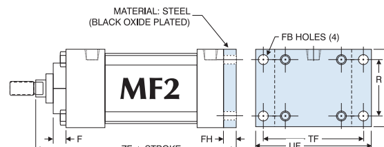
1.50" - 6.00" BORES
