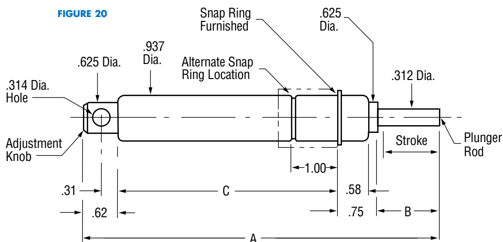
KINECHEK CUSHION-START AND SLOW RETURN
