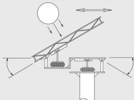
SOLAR TRACKER
