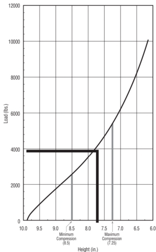
LOAD/DEFLECTION CURVE
