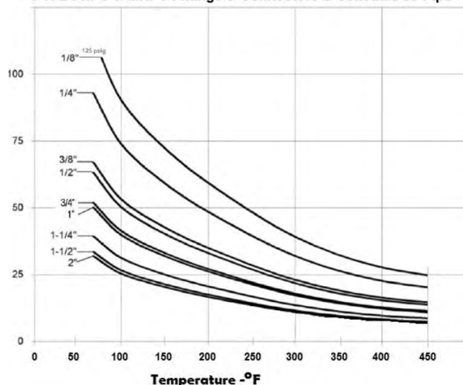
IPS Pressure Ratings PTFE FNPT & MNPT Fittings & Connectors & Schedule 80 Pipe
