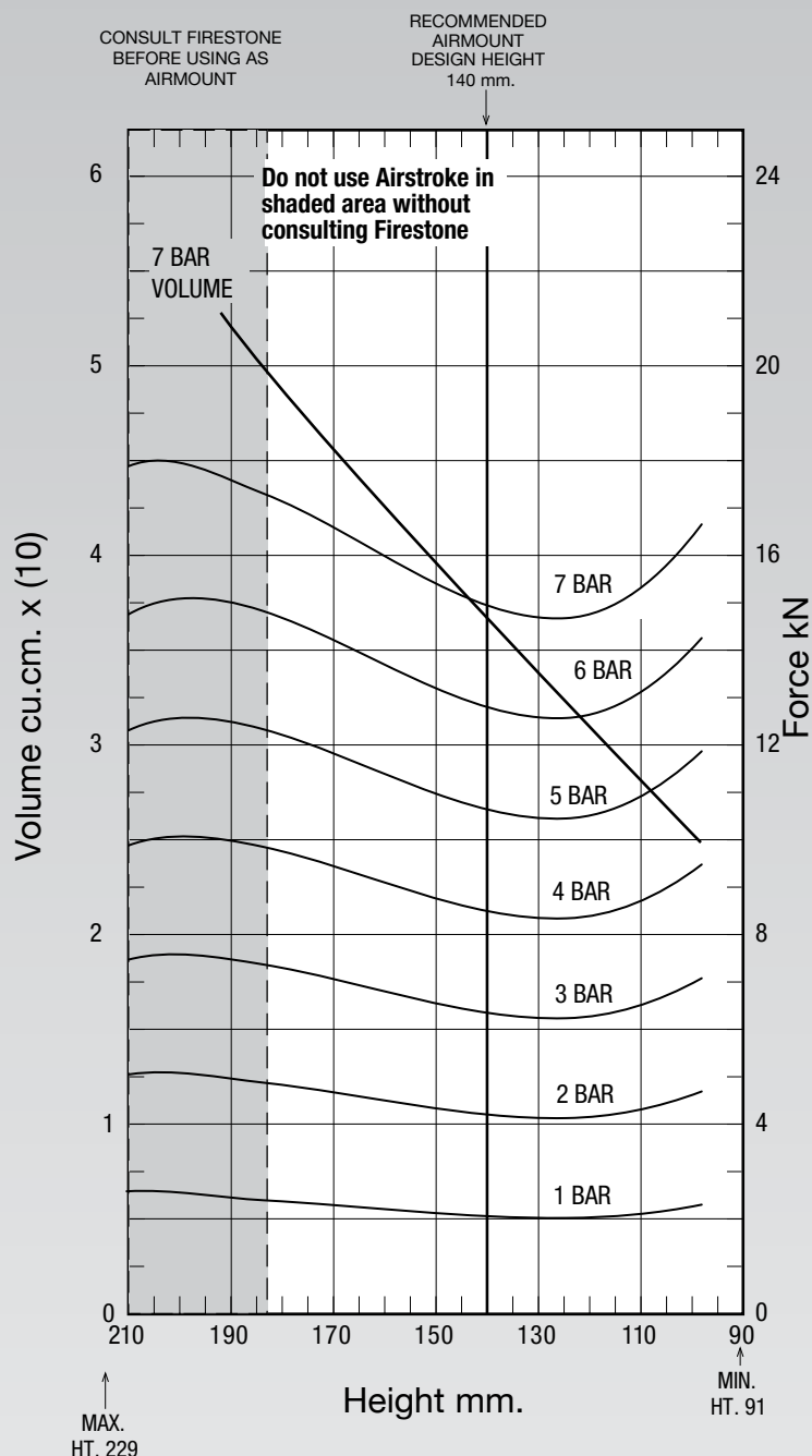
Force Table (Use for Airstroke™ actuator design)
