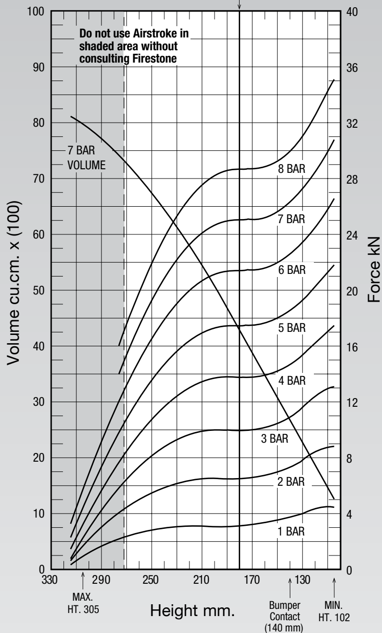
Force Table (Use for Airstroke™ actuator design)
