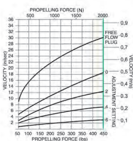
Tension Mode Adjustment Setting Curve
