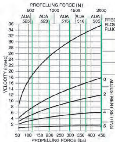
Compression Mode Adjustment Setting Curve
