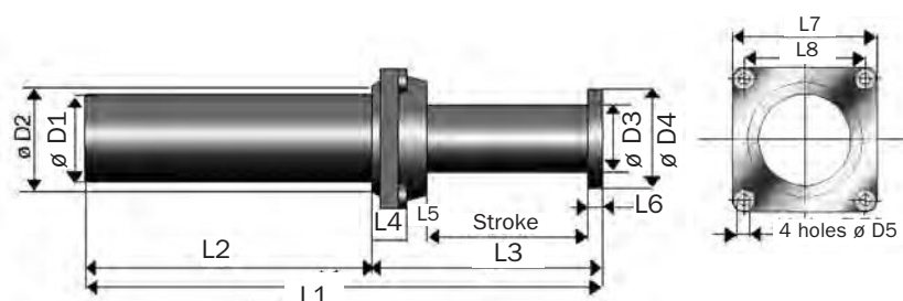
XLR Series - Front Flange Mount- Fc
