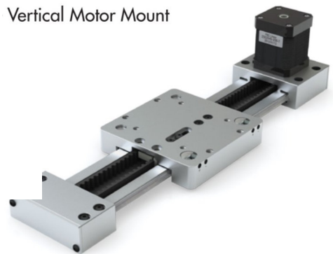
Vertical Motor Mount
