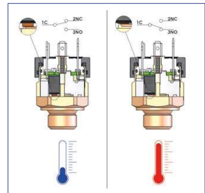
FIG. 3 Contatti in scambio (SPDT) Switching contacts (SPDT)
