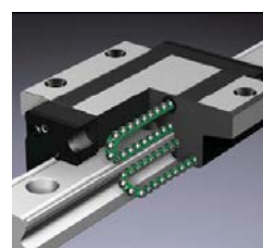
Grease pocket
