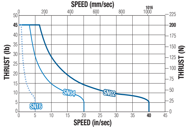
MXE16: PV Limits: Acme Screws
