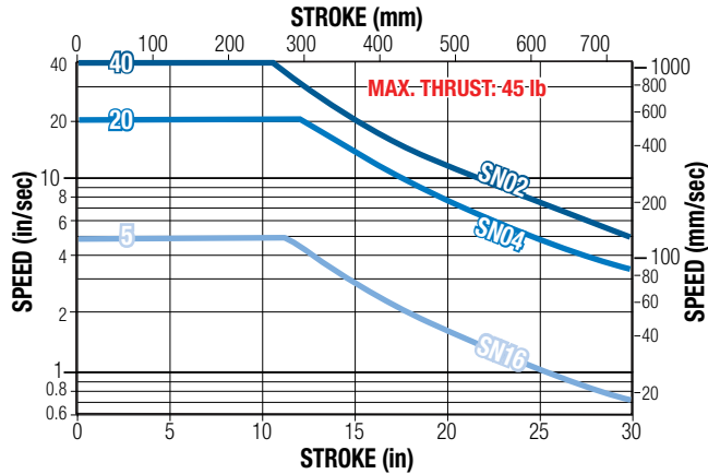
MXE16: Critical Speed: 0.250" ACME
