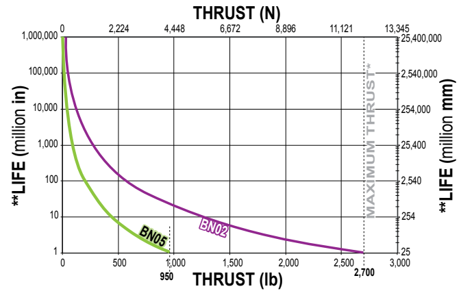
MXE50: Life: Ball Screw
