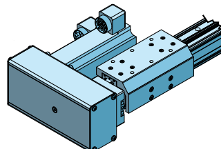
REVERSE-PARALLEL LEFT (RPL) mounting surface shown UP SIDE MOUNT (Left Shown)
