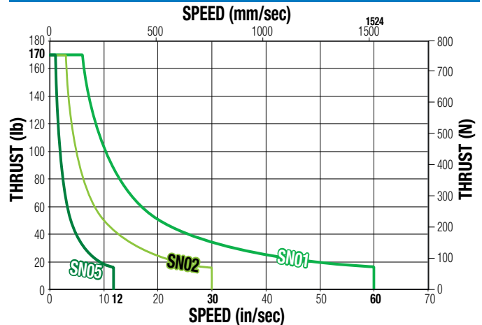
MXE40: PV Limits: Acme Screws
