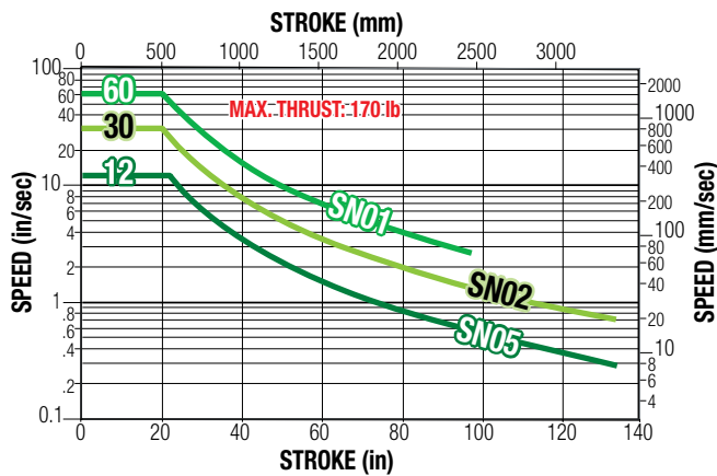
MXE40: Critical Speed: 0.625" & .75" ACME
