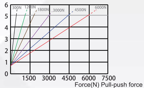
CURVE(Force/ current)
