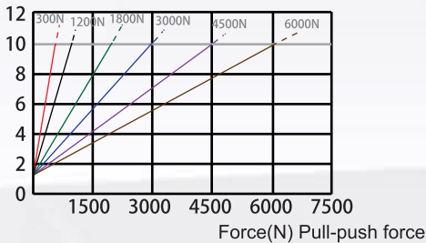
CURVE(Speed/force)
