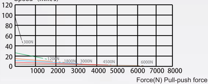
CURVE(Speed/force)
