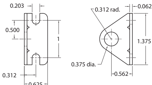
FB-0891 Foot Bracket Material: Steel, bright zinc plated
