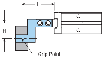
EXTERNAL GRIP
