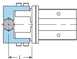
EXTERNAL GRIP
