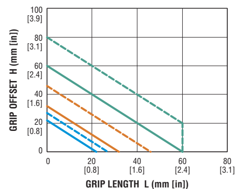
OGZD15-20x10 INTERNAL GRIP
