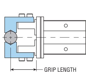
EXTERNAL GRIP
