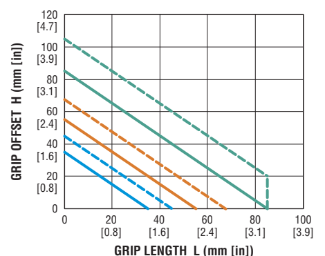
OGZD15-25x14 INTERNAL GRIP
