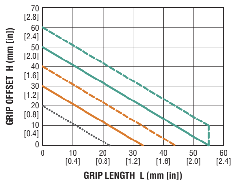
OGZD15-16x6 EXTERNAL GRIP
