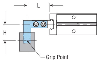
INTERNAL GRIP
