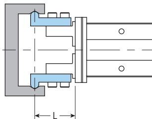
INTERNAL GRIP
