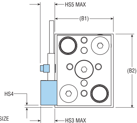
CLOSED POSITION
